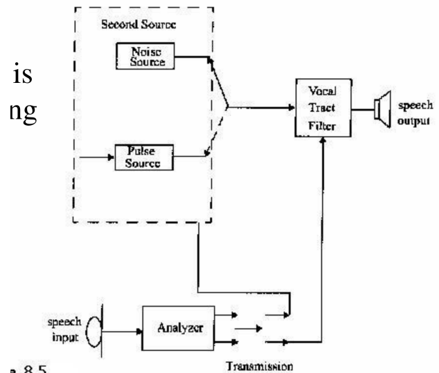
Fig 8.5 Speech generation model.
