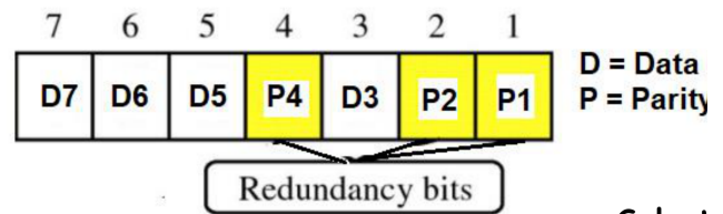
Fig : 7 bit Hamming code
