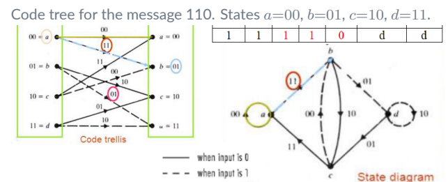
Code trellis and the equivalent state diagram. Solid line = input 0, dashed = input 1.
