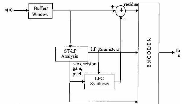
Figure 8.9 Block diagram of a RELPC encoder.
